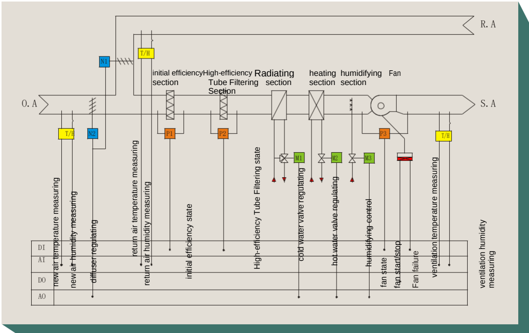
Air Conditioning System with High-efficiency Tube
