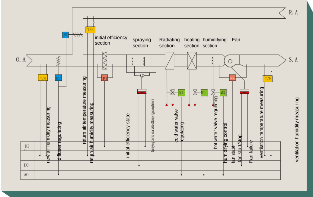
Air Conditioning System with Spraying Section
